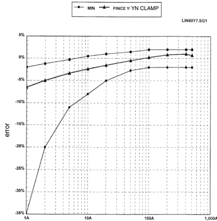
Error on measurement at 50 Hz
